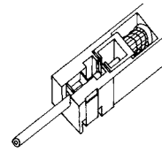
Bowden cable locked into assembly
